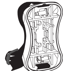
Punch-Down-Terminating Puck
