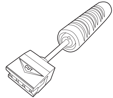
Category 6 110 Style Multi Pair Termination Tool
