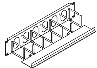
2U Through-the-Rack Panel Dimensions: 89mm x 483mm x 102mm (3.5"H x 19"W x 4"D) Shipping Weight: 588g (1 lb. 5 oz.)
