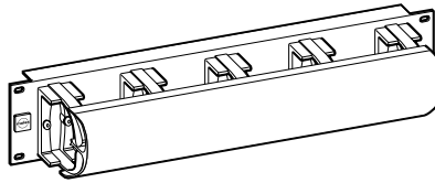
2U Ring Run Panel with Cover Dimensions: 89mm x 483mm x 64mm (3.5"H x 19"W x 2.6"D) Shipping Weight: 1064g (2 lb. 6 oz.)
