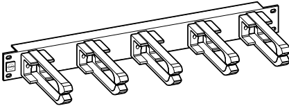
1U Deep Ring Run Dimensions: 44mm x 483mm x 127mm (1.75"H x 19"W x 5"D) Shipping Weight: 728g (1 lb. 10 oz.)
