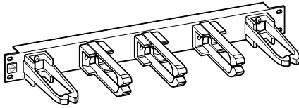
1U Deep Horizontal/Vertical Ring Run Dimensions: 44mm x 483mm x 127mm (1.75"H x 19"W x 5"D) Shipping Weight: 728g (1 lb. 10 oz.)
