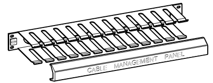
1U Cable Management Panel Dimensions: 44mm x 483mm x 74mm (1.75"H x 19"W x 2.9"D) Shipping Weight: 588g (1 lb. 5 oz.)
